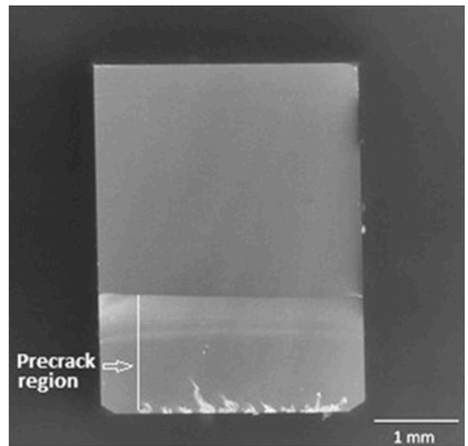
Fig. 7. Example of the fracture surface of a glass-ceramic specimen after the 3-point bending fracture stage. The pre-crack region is clearly visible at the bottom, as well as the pre-crack arrest line standing as the frontier to the fast crack extension region (upper region). The glass-ceramic was obtained after heat treatment for 48 h at 1006 K and 153 min at 900 °C.
