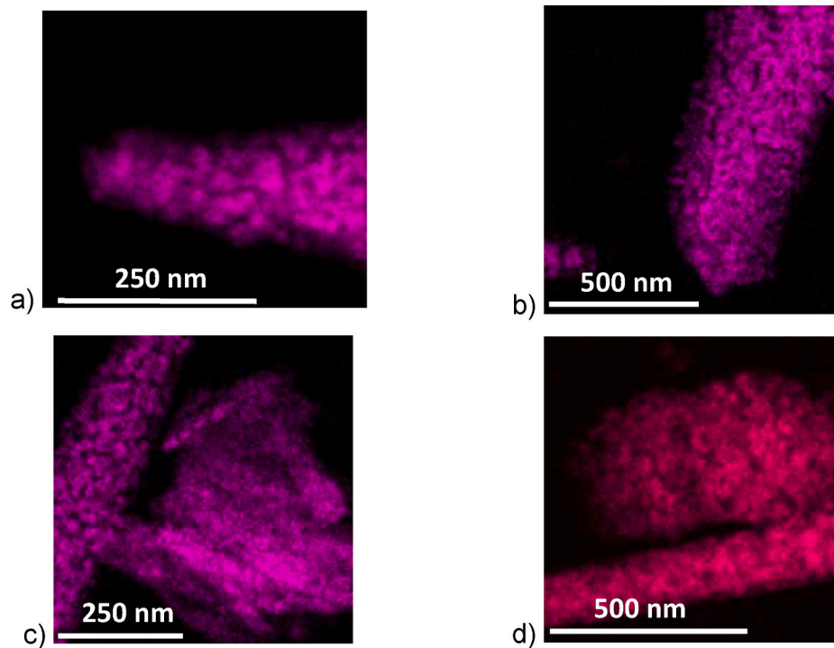
Fig. 12. Evolution of Al distribution in the glass-ceramics obtained after a nucleation step of 48 h at 733 °C and a growth treatment at 900 °C for: a) 31 min. b) 61 min c) 92 min. d) 153 min.
