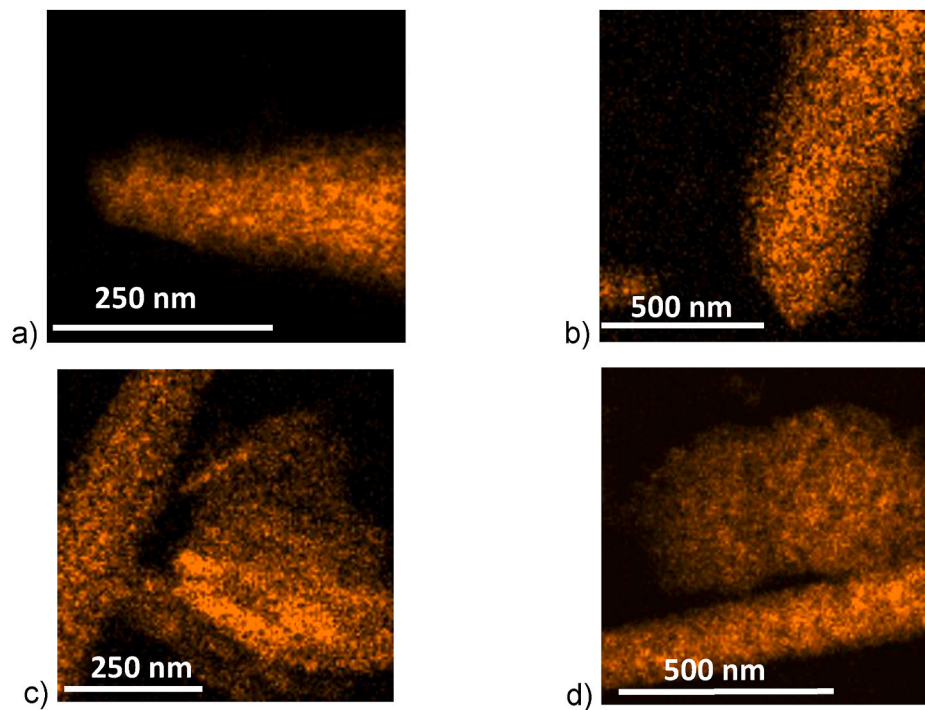
Fig. 10. Evolution of Mg distribution in the glass-ceramics obtained after a nucleation step of 48 h at 733 °C and a growth treatment at 900 °C for: a) 31 min. b) 61 min c) 92 min. d) 153 min.
