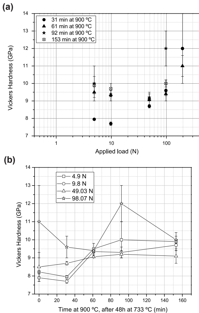
Fig. 6. a) Hardness for different loads for glass-ceramic samples and b) hardness versus crystal growth time at 900 °C, after 48 h at 733 °C, for different loads. Error bars represent the standard deviation of at least five imprints.
