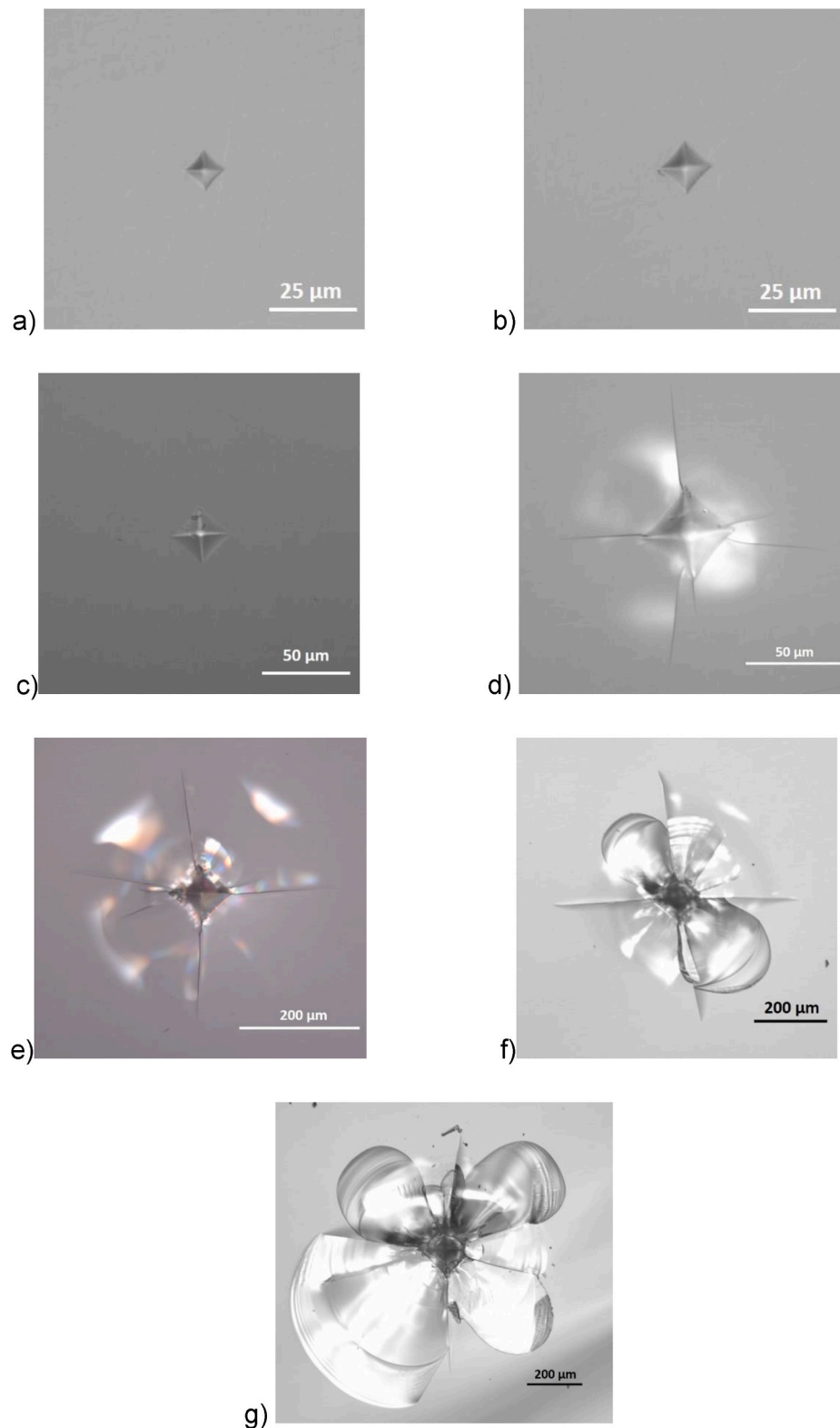
Fig. 3. Vickers indent performed on parent glass samples. a) 600 mN; b) 1 N; c) 4.9 N; d) 9.8 N; e) 49.03 N; f) 98.07 N and g) 196.1 N.
