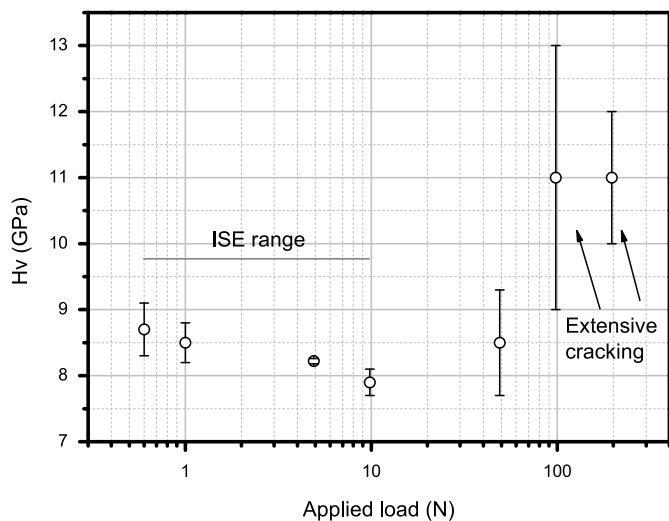
Fig. 4. Vickers hardness as a function of the applied load for the glass sample of the composition shown in Table 1. The range of ISE (Indentation Size Effect) is shown.
