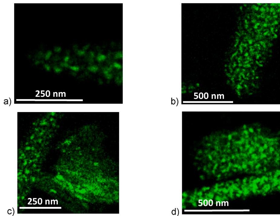
Fig. 11. The evolution of Ti distribution in glass-ceramics obtained after a nucleation step of 48 h at 733 °C and a growth treatment at 900 °C for: a) 31 min. b) 61 min c) 92 min. d) 153 min.
