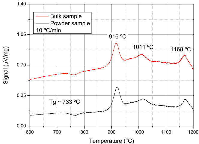
Fig. 2. DSC traces of the studied composition. Adapted from Ref. [14].
