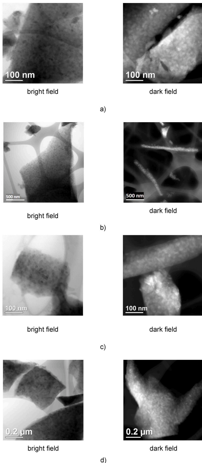
Fig. 9. STEM-images in bright and dark field modes of glass-ceramics obtained after nucleation treatment at 48 h at 733 °C and growth treatment of a) 31 min at 900 °C; b) 61 min at 900 °C; c) 92 min at 900 °C and d) 153 min at 900 °C.
