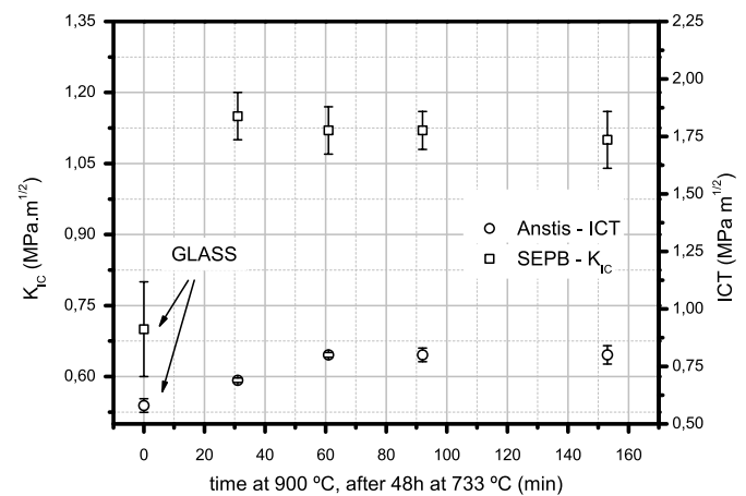
Fig. 8. K_{IC} values obtained by Single Edge Pre-cracked Beam (SEPB) and indentation cracking (ICT) resistance using the Anstis equation (19), for the precursor glass and glass-ceramics obtained after different crystal growth periods at 900 °C.
