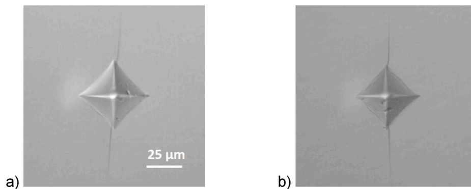
Fig. 5. Indent profile for different applied loads in the investigated MAS glass-ceramics obtained for the same nucleation treatment (48 h at 733 °C) and crystal growth treatments at 900 °C for: a) 31 min; b) 61 min; c) 92 min d) 153 min. The scale is the same for all images obtained under the same load.
