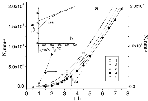
Fig. 5. (a) Number density of \text{Li}_2\text{O}\cdot 2\text{SiO}_2 crystals developed at T_d = 530 \text{ }^\circ\text{C} (curves 1 and 5), 560 \text{ }^\circ\text{C} (curve 2), 594 \text{ }^\circ\text{C} (curve 3), and 626 \text{ }^\circ\text{C} (curve 4) as a function of nucleation time at T_n = 453 \text{ }^\circ\text{C} [38]. (b) Induction time versus development temperature.
