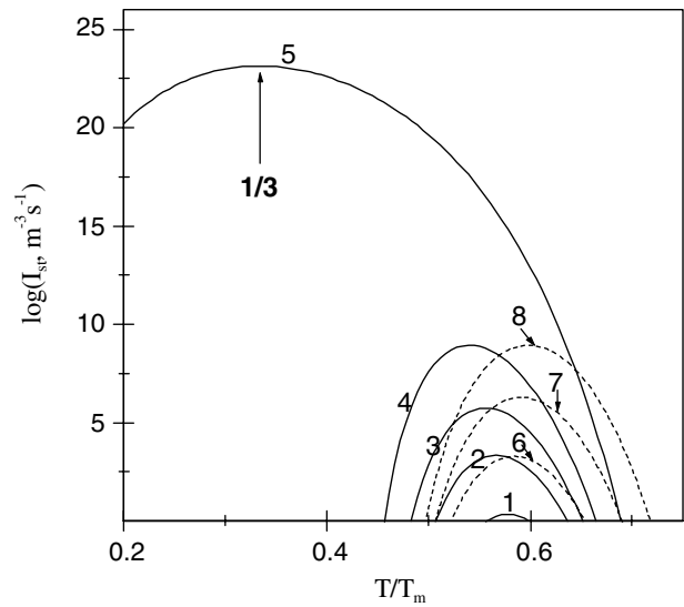
Fig. 12. Temperature dependence of homogeneous nucleation rates. The curves were calculated with Eqs. (1), (30), and (32) with a pre-exponential term I_o = 10^{42} \text{ m}^{-3} \text{ s}^{-1} and following values of the parameters characterizing the temperature independent parts of the thermodynamic ( C_1 ) and kinetic ( C_2 ) barriers: C_1 = 6.5 (curves 1–5), 5.8 (curve 6), 5.1 (curve 7), 4.5 (curve 8); C_2 = 6 (curves 1 and 6–8), 4.8 (curve 2), 3.9 (curve 3), 2.8 (curve 4), 0 (curve 5).
