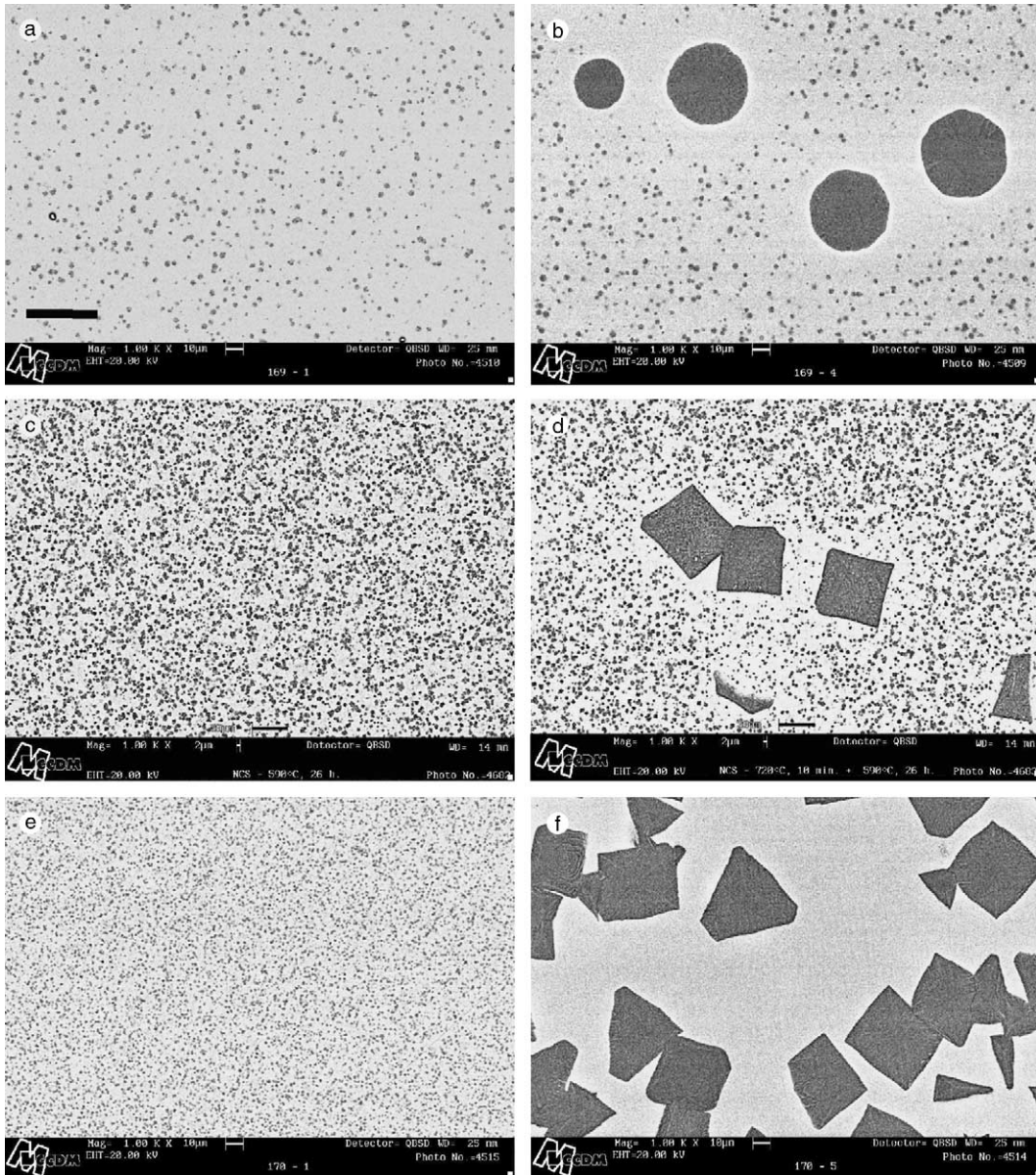
Fig. 15. SEM micrographs of glasses N1, N4 and N5 subjected to single (a, c, e) and double stage (b, d, f) heat treatments. Single stage: T_{n-g} , t_{n-g} ; double stage: T_{gr} , t_{gr} + T_{n-g} , t_{n-g} ; T_{n-g} = 590 °C; t_{n-g} = 1340 min (a), 1560 min (c), 2140 min (e). T_{gr} = 700 °C (b), 720 °C (d, f); t_{gr} = 40 min (b), 10 min (d), 20 min (f). Bar denotes 50 \mu m.
