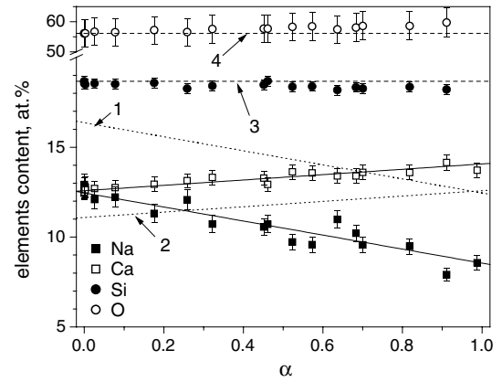
Fig. 11. Composition of glass N4, measured by EDS (points), and of crystals calculated from the parent glass composition (dotted lines 1 and 2 – Na and Ca, respectively) versus volume fraction crystallized at T = 650 °C. Solid lines fit the experimental data. Dashed lines 3 (Si) and 4 (O) correspond to the parent glass composition.
